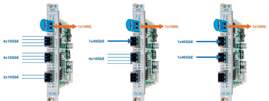
Figure 1: 10GbE and 40GbE service aggregation configurations using PM 100G-EMUX
